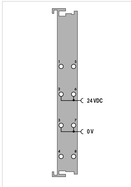
Figure: 750-602/040-000
