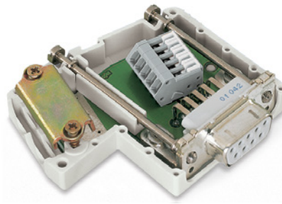
Figure: 750-961
