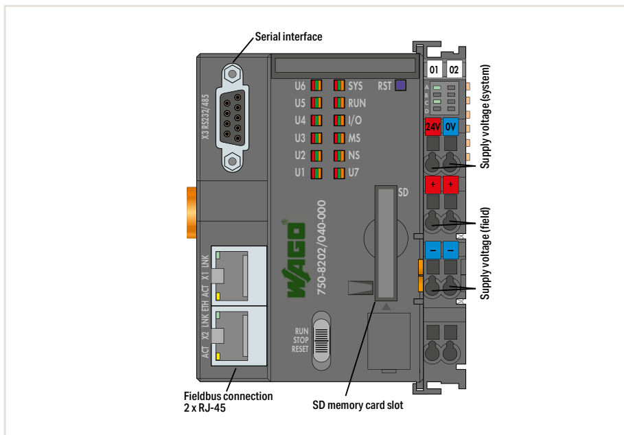
Figure: 750-8202/040-000
