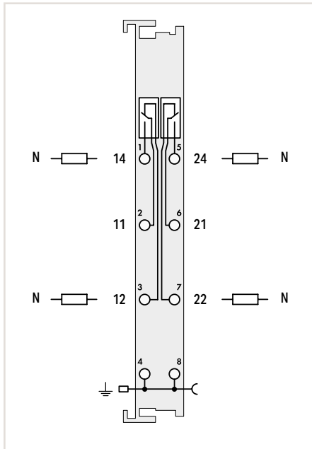
Figure: 750-514
