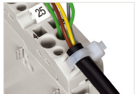
Securing a cable to the connector.
