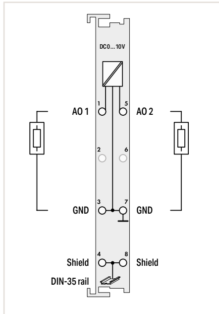
Figure: 750-550
