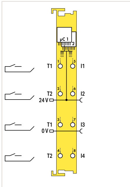
Figure: 750-661/000-003
