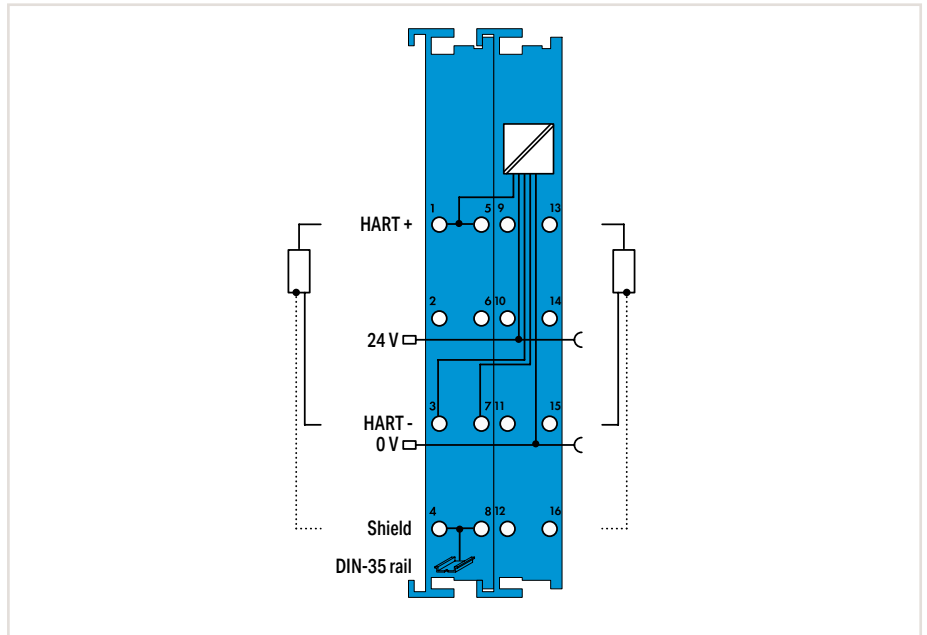
Figure: 750-484
