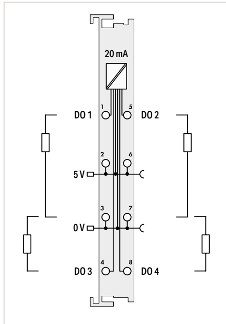
Figure: 750-519
