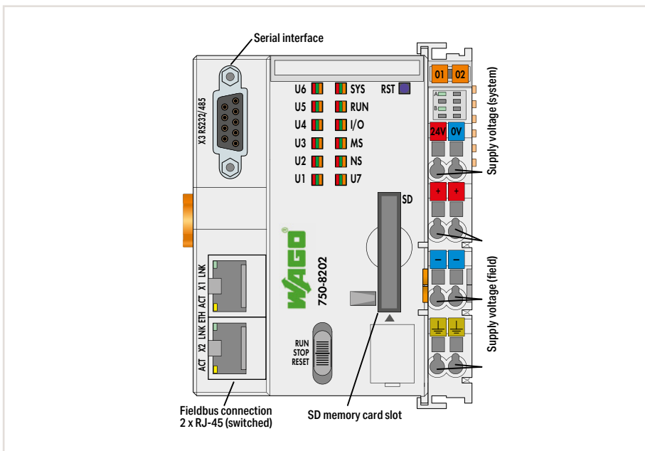
Figure: 750-8202
