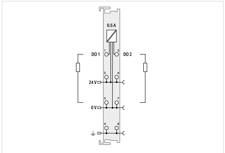
Figure: 750-501
