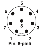
Pin, 8-pinli
